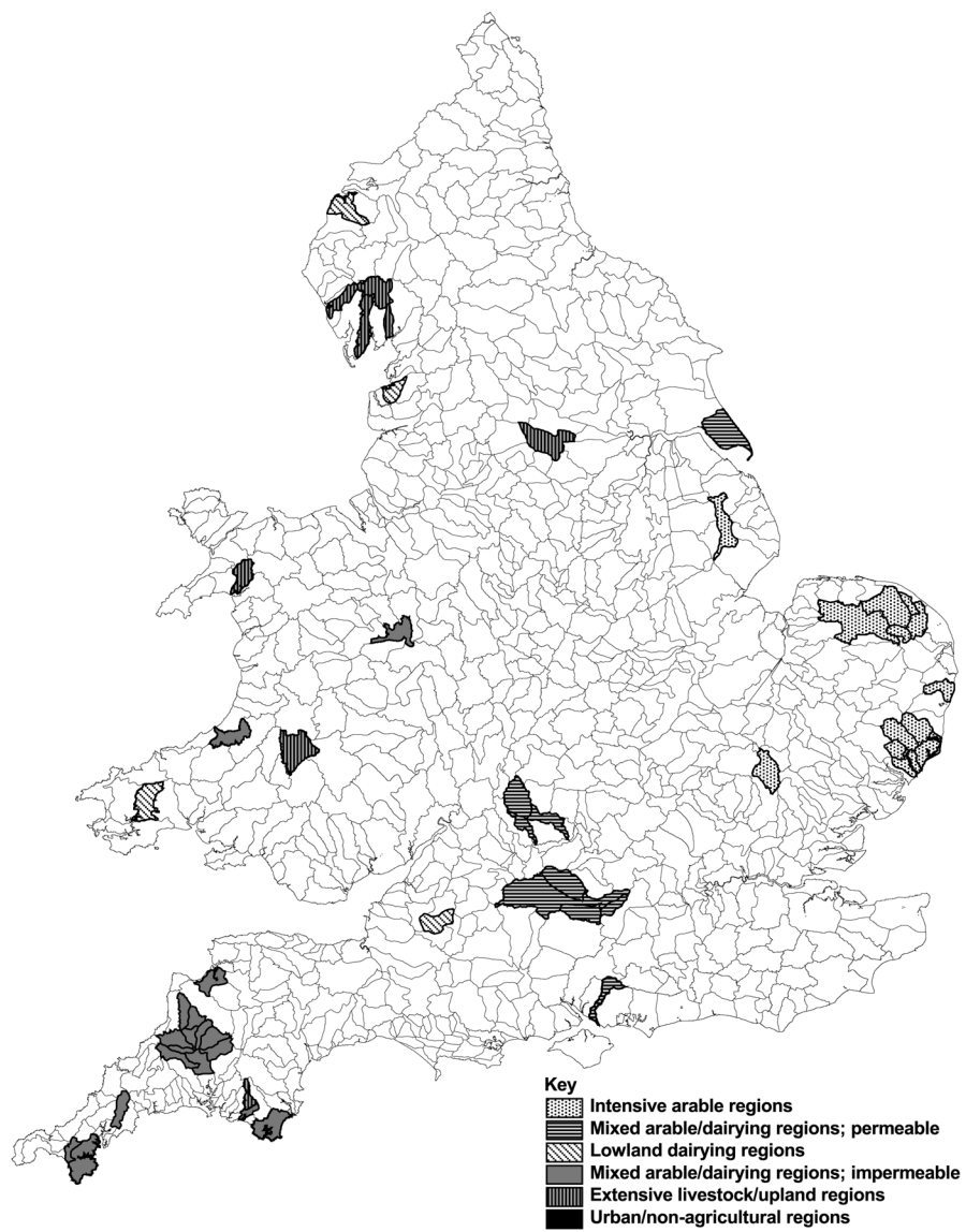
Figure 2. Export coefficient modelling applications to surface water catchments in England and Wales.
